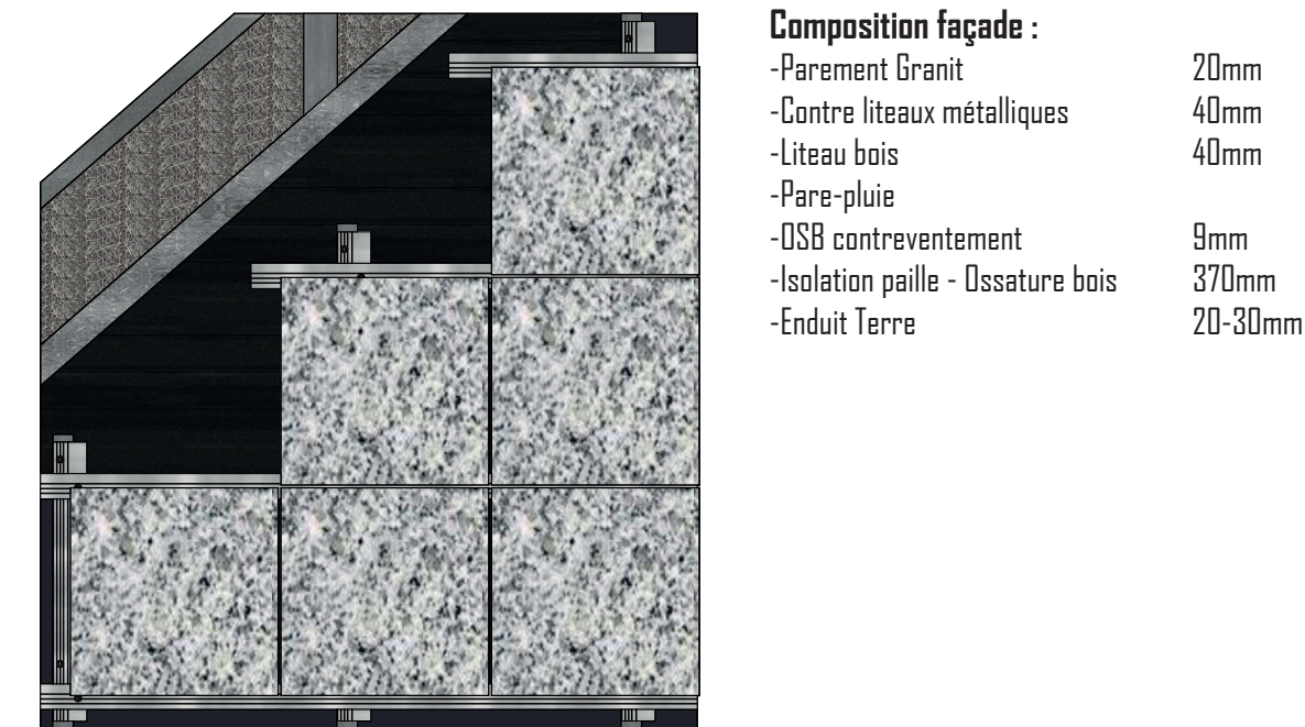
ELEVATION DETAIL FACADE 1: 20EME
